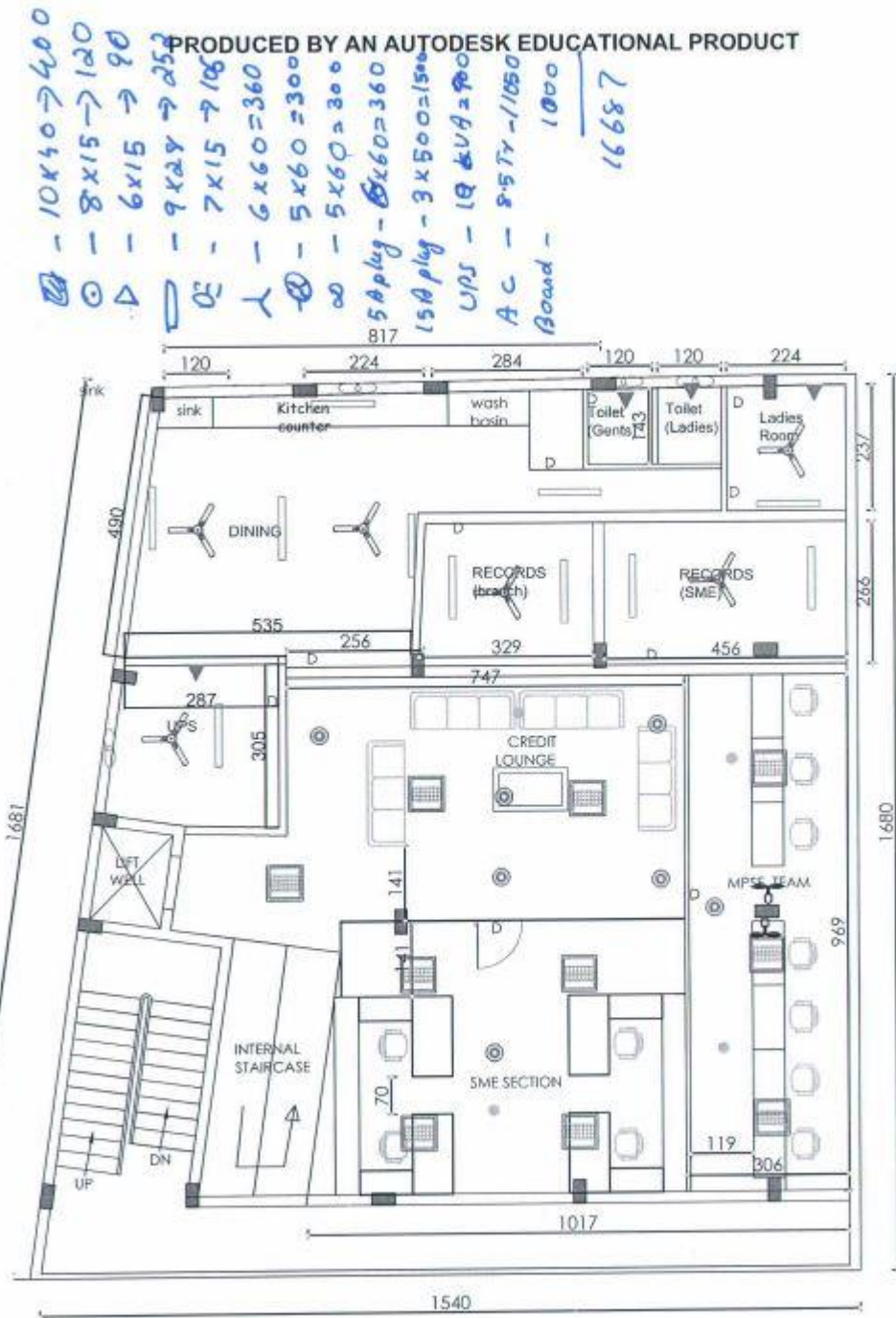
SBI PALLIPPURAM - FIRST FLOOR -DWG NO.6 DT. 30.12.23
